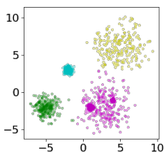
Clustering
