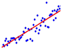
Regression
