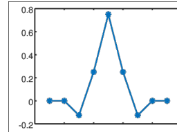
Low-level Filter
